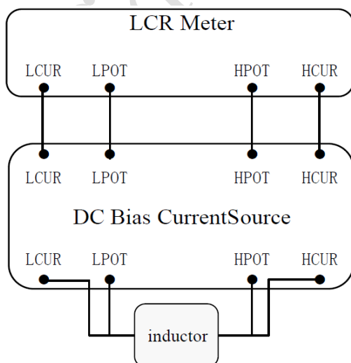
Isat test schematic diagram
